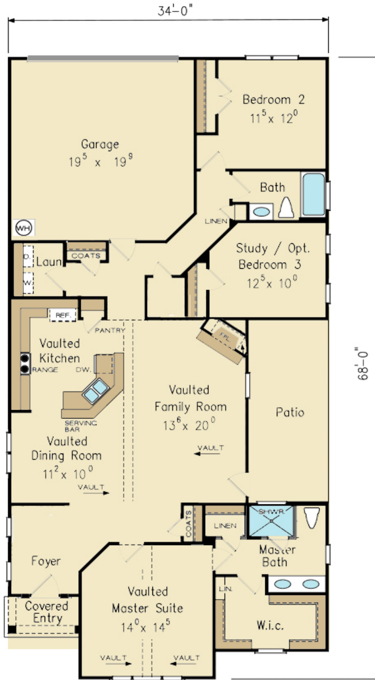
FLOOR PLAN
