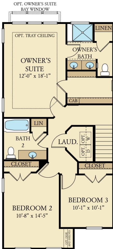
UPPER FLOOR
